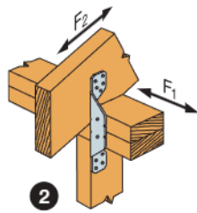
2 H2A Installation
