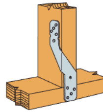
12 H8 attaching Stud to Sill (4) 0.131" x 2½" nails into plate, (5) 0.131" x 2½" nails into stud, refer to footnote 3 for loads)
