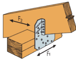
15 H10A Installation
