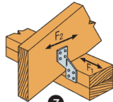
7 H3 Installation (nails into upper top plate)
